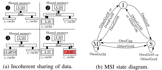
Fig. 1: Cache coherence.
